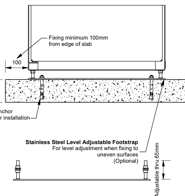
Installation using Stainless Steel Level Adjustable Footstrap
