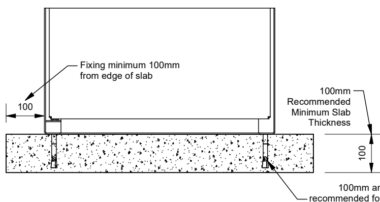
Installation without Stainless Steel Level Adjustable Footstrap
