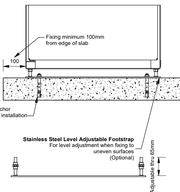
Installation using Stainless Steel Level Adjustable Footstrap
