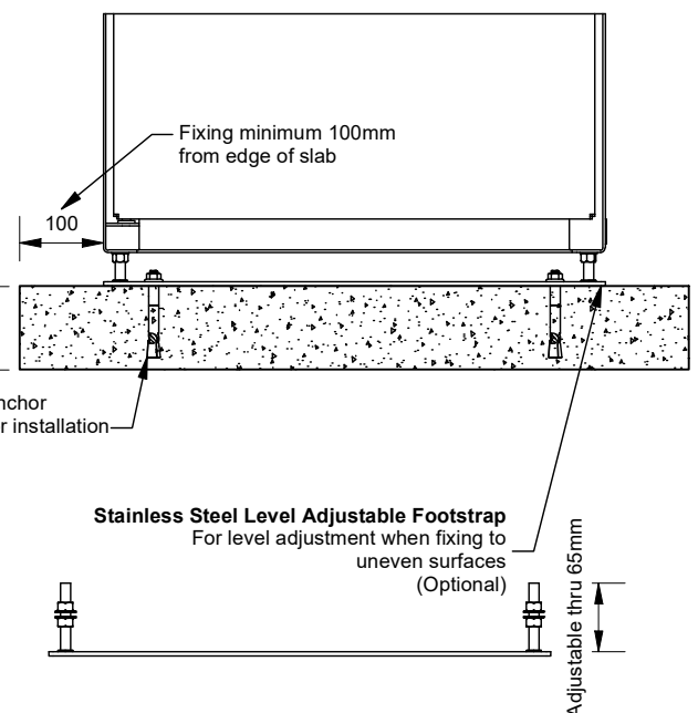
Installation using Stainless Steel Level Adjustable Footstrap
